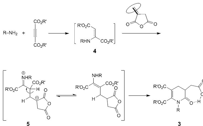
Scheme 2. Mechanistic Proposal for the Synthesis of 2-[1-Alkyl-5,6-bis(alkoxycarbonyl)-1,2,3,4-tetrahydro-2-oxopyridin-3-yl]acetic Acid Derivatives 3a–3i
